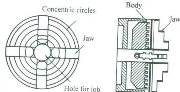
Four Jaw Independent chuck
