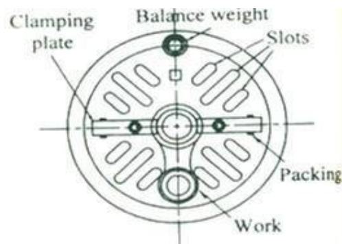
Face Plate
