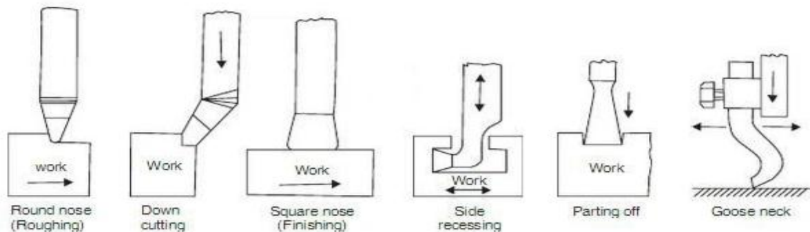
CUTTING TOOLS
